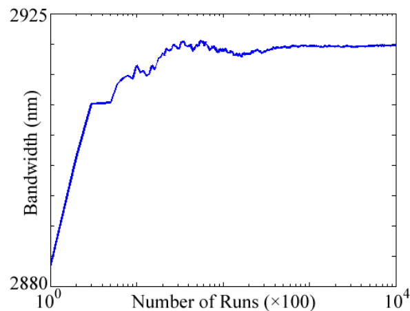
Fig. 10. Average bandwidth versus number of samples in the ensemble average.
