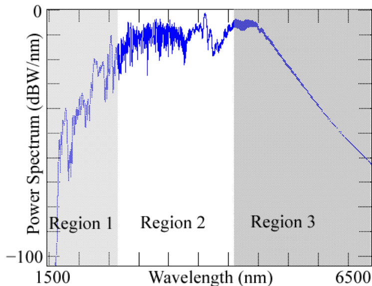
Fig. 2. Example supercontinuum spectrum showing three regions.
