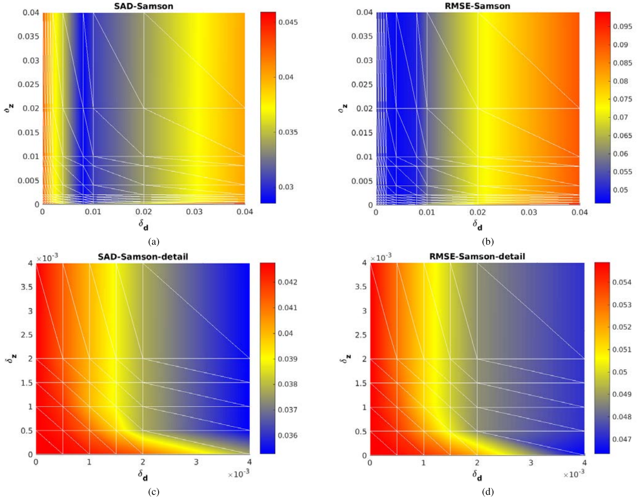
Fig. 10. SAD (a), (c) and RMSE (b), (d) assessment for Samson dataset using different sparsity factors. Note that (c) and (d) figures provide a detail of (a) and (b) ones, respectively.
