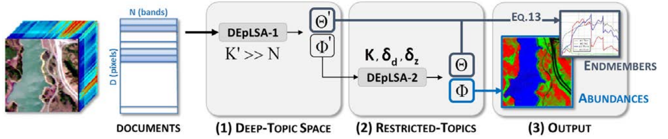
Fig. 4. Overview of the proposed HU framework.
