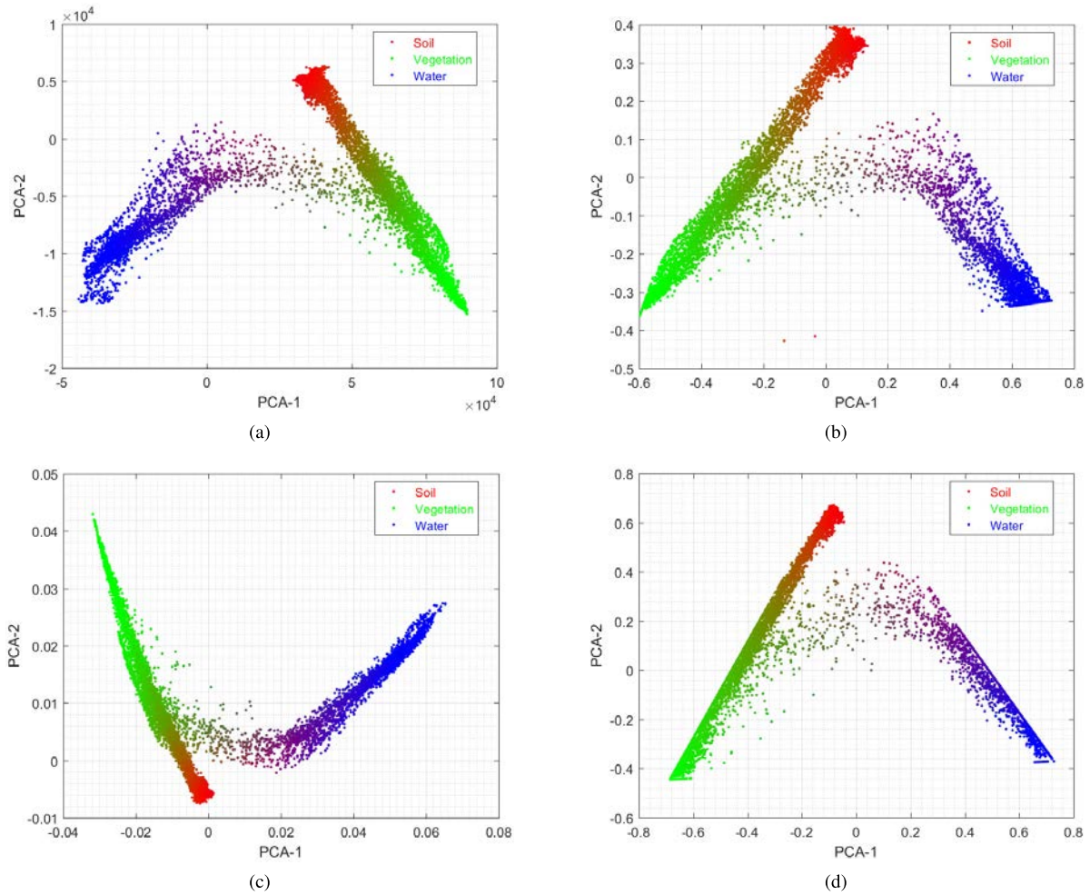
Fig. 11. Visual representation of Samson data projected onto the two first PCA components. (a) Original spectral space. (b) pLSA-sp space. (c) Deep topic space. (d) Restricted topic space.
