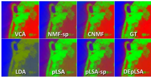
Fig. 6. Samson abundance results for VCA, NMF-sp, CNMF, LDA, pLSA, pLSA-sp, and the proposed DEpLSA method. Top-right position: ground-truth (GT) image. Pure red: soil endmember. Green: tree endmember. Blue: water endmember.
