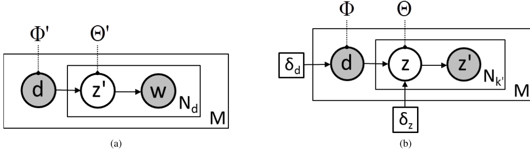
Fig. 3. Two-phase model relaxation for the proposed DEpLSA model. See Fig. 2 for notation details. (a) DEpLSA-1, first-phase model relaxation. (b) DEpLSA-2, second-phase model relaxation.
