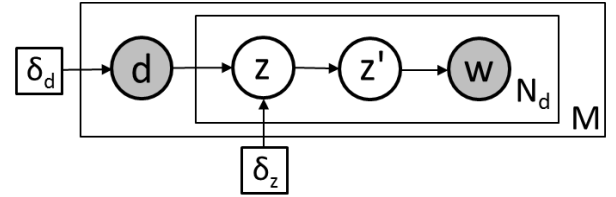
Fig. 2. Proposed DEpLSA topic model. Nodes d , z , z' , and w : document, restricted-topic, deep-topic, and word random variables. N_d : number of words in d and M is the total number of documents in the collection. \delta_d and \delta_z : sparsity factors for documents and restricted topics, respectively.
