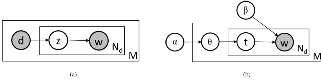
Fig. 1. (a) pLSA topic model. (b) LDA topic model. Nodes d , z , and w : document, topic, and word random variables. \alpha and \beta : Dirichlet hyperparameters for the topic-document and word-topic distributions. \theta : multinomial distribution generated from the corresponding Dirichlet prior \alpha and t corresponds to the categorical distribution used for the topic activations. N_d and M : number of words in the document and the total number of documents in the collection. Shaded nodes: observable variables of the models.
